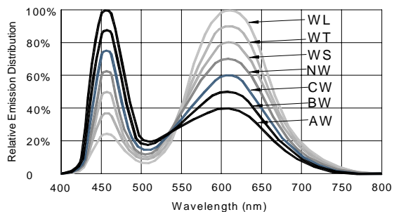
Wavelength Characteristics
